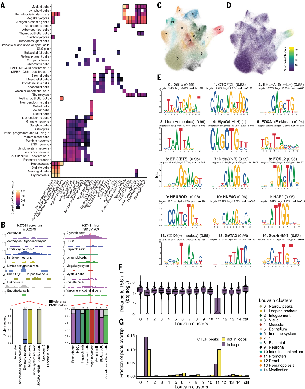
Fig. 5. Heritability enrichment and coaccessibility of candidate regulatory regions.
